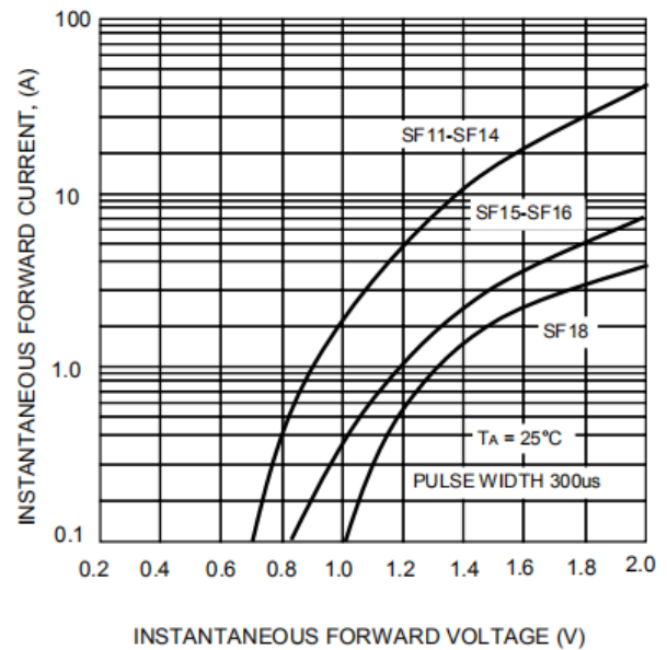
FIG.2-TYPICAL FORWARD CHARACTERISTICS
