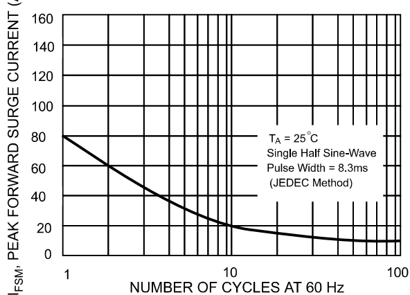
Fig.1-MaximumPeakForwardSur ge Current (per leg)
